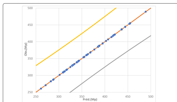
Figure 4: Correlations of observed and predicted Mp calculated using ANN.
