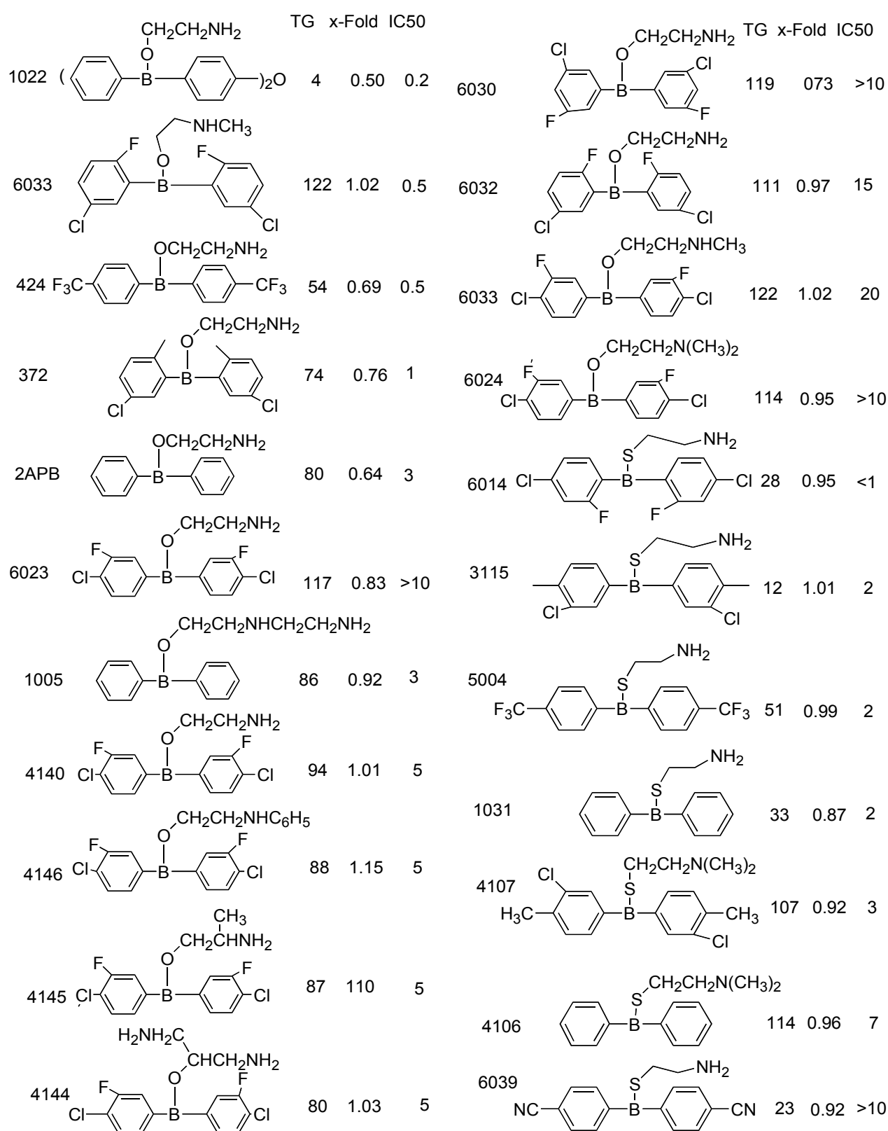
Figure 2: Amino alcohol adduct compounds & Aminothioli adduct compounds.
