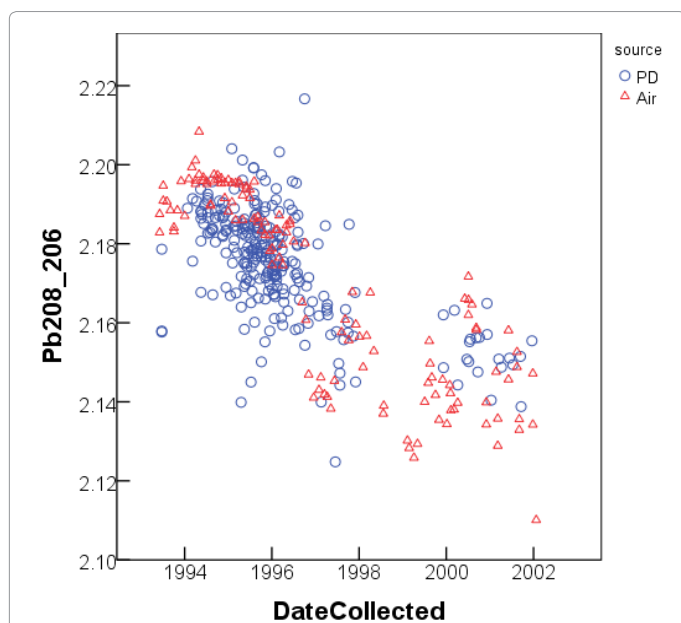
Figure 1: Measured ^{208}\text{Pb}/^{206}\text{Pb} ratios versus Date sampled for air filters and petri dish dust.
