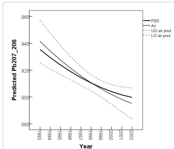
Figure 5: Predicted ^{207}\text{Pb}/^{206}\text{Pb} ratios versus Date sampled for air filters and PDD. The bold solid line is the curve fitted to the PDD measurements, the bold dotted line is the curve fitted to the air measurements and the light dashed lines are the upper and lower 95% confidence intervals for the prediction of the air measurements from the PDD measurements, derived as described above.
