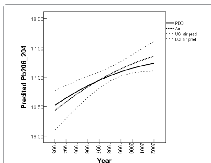
Figure 6: Predicted ^{206}\text{Pb}/^{204}\text{Pb} ratios versus Date sampled for air filters and PDD. The bold solid line is the curve fitted to the PDD measurements, the bold dotted line is the curve fitted to the air measurements and the light dashed lines are the upper and lower 95% confidence intervals for the prediction of the air measurements from the PDD measurements, derived as described above.
