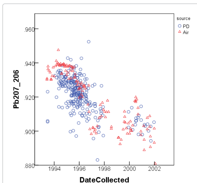
Figure 2: Measured ^{207}\text{Pb}/^{206}\text{Pb} ratios versus Date sampled for air filters and petri dish dust.
