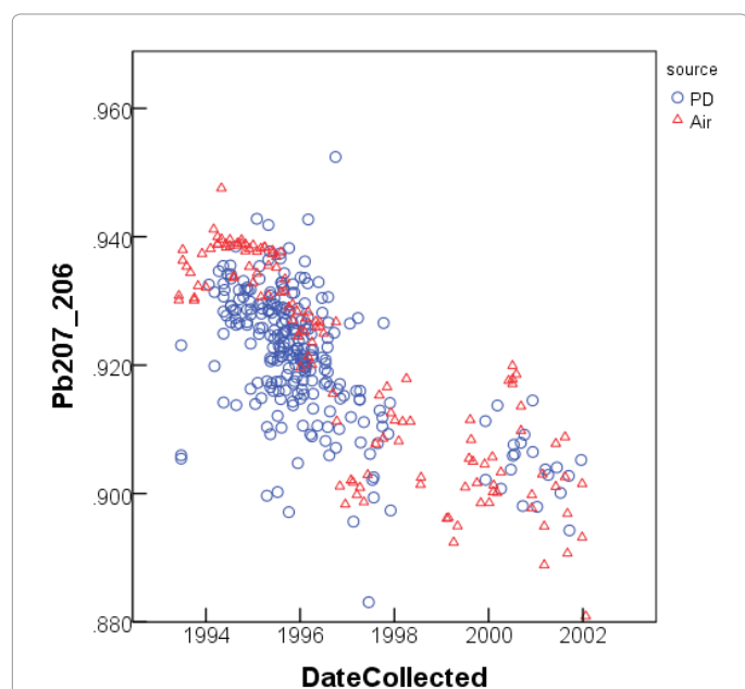
Figure 2: Measured ^{207}\text{Pb}/^{206}\text{Pb} ratios versus Date sampled for air filters and petri dish dust.
