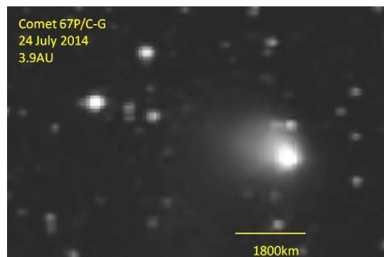
Figure 1: July 24, 2014, Image of Comet 67P/C-G at 3.9AU showing dust/gas coma and tail (Courtesy, OSIRIS/ESA).
