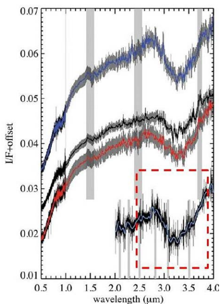
Figure 6: Reflectance spectra of 3 regions of the surface. The boxed curve is to be compared with reflectance/transmittance spectra of candidate materials (Capaccione et al. [5]).
