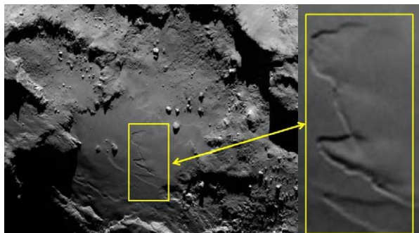
Figure 2: Rosetta imaging of Comet 67P/C-G. Left: The 600 x 800 m Cheops 'sea'. The image shows it curving away into shadow approaching the terminator at bottom left. The plateau at the top right corner (semi-circular) is a few 100 m higher than the sea and appears to have shed debris at the cliff-foot. Right: Enlargement of the major fissure, ~10 m deep and 10-20 m wide. (ESA/Rosetta/MPS for OSIRIS Team).
