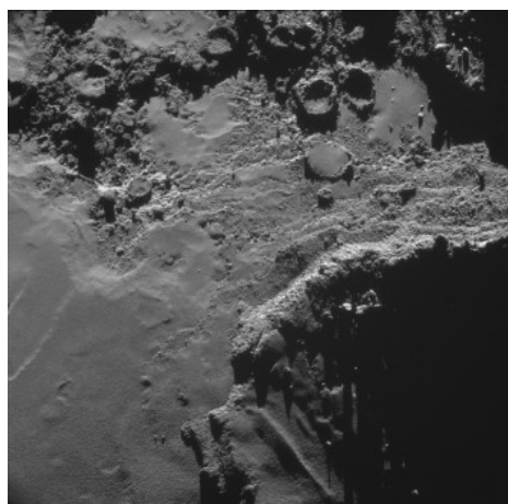
Figure 3: Flat-bottomed impact craters, showing impact-melt interiors that could be re-frozen lakes ~40 m across. The left of the image shows the corner of the Cheops sea to the upper right of the Cheops boulder cluster.
