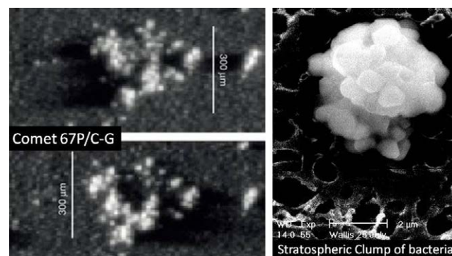
Figure 8: Coarse (14 micron resolution) image of disintegrating cometary dust clump (L) compared with a clump of stratospheric particles, (Wallis et al. [7]) recovered from a height of 41 km.
