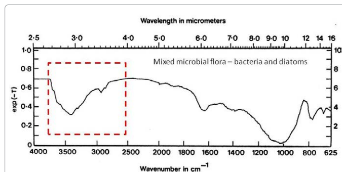
Figure 7: Transmittance curve for a mixed microbial flora (bacteria and diatoms) from a sample of water from the River Taff, Cardiff. (Experiments conducted by Al-Mufti [5]).
