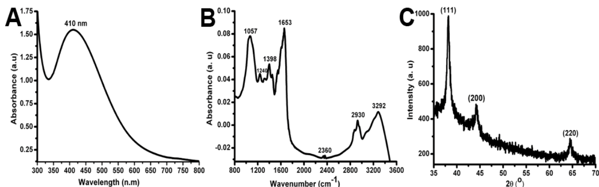
Figure 2: UV-Vis, FTIR and XRD measurements of the as-prepared parent silver nanoparticle suspension. (A) UV-Vis spectrum of the as-prepared parent silver nanoparticles showing a broad peak indicating the presence of anisotropic silver nanoparticles. (B) Fourier transform spectra of the as-prepared silver nanoparticles, significant vibration bands are labeled. (C) XRD analysis of the as-prepared silver nanoparticle powder.
