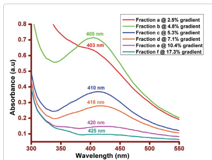
Figure 4: UV-Vis spectroscopy measurements of the various pooled fractions a, b, c, d, e and f sedimented at sucrose gradients of 2.5%, 4.8%, 5.3%, 7.1%, 10.4% and 17.3% respectively. The individual samples and their surface plasmon peak are labeled.
