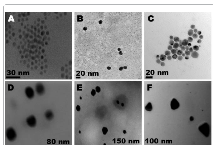
Figure 5: Transmission electron microscopy images of the various pooled fractions; A, B, C, D, E and F upon sedimentation using sucrose density gradient at 2.5%, 4.8%, 5.3%, 7.1%, 10.4% and 17.3% respectively, following separation of the anisotropic silver nanoparticles.
