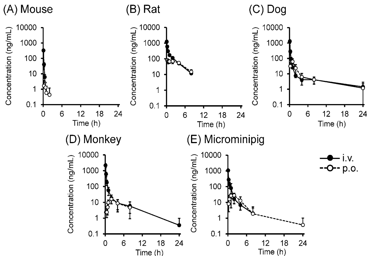
Figure 2: Plasma concentration of losartan in mice (A), rats (B), dogs (C), monkeys (D), and microminipigs (E) after the single intravenous and oral administration of 5 mg losartan. Each point and bar is represented as the mean \pm S.D. of three animals.
