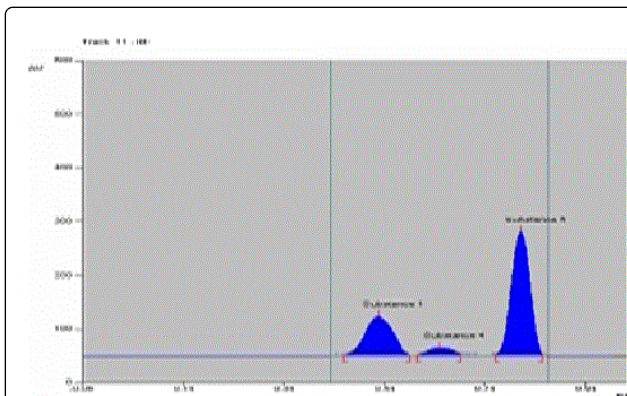
Figure 13: Acid forced degradation chromatogram of AGO by RP-TLC method.
