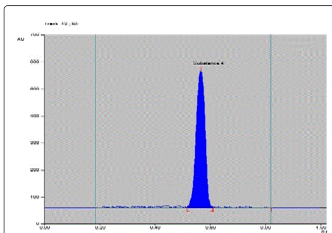
Figure 2: 2D Chromatogram of AGO ( R_f=0.58 \pm 0.04 ) using Ethyl acetate: MeOH:Amm. (33%) (85:10:5, v/v/v) as mobile phase at 230 nm by NP-TLC method.
