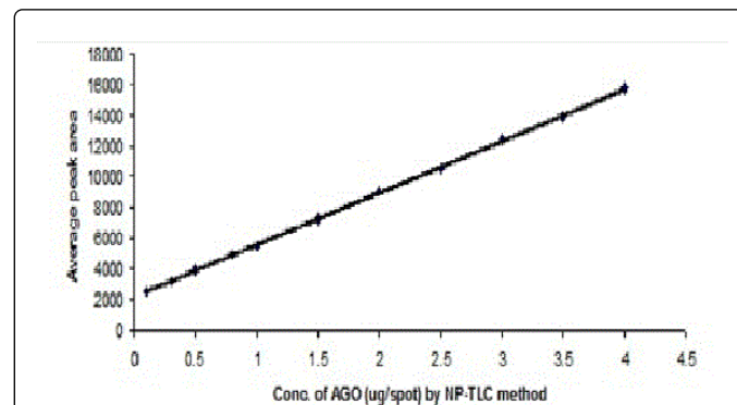
Figure 8: Calibration curve for NP-TLC method of AGO.
