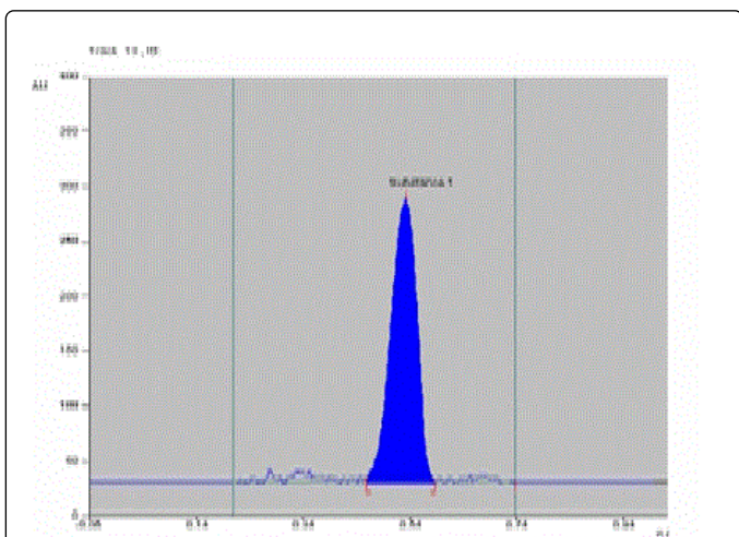
Figure 4: 2D chromatogram of AGO ( R_f=0.54 \pm 0.02 ) using 0.1% TEA: Acetonitril (60:40, v/v) PH=2 as mobile phase at 280 nm by RP-TLC method.
