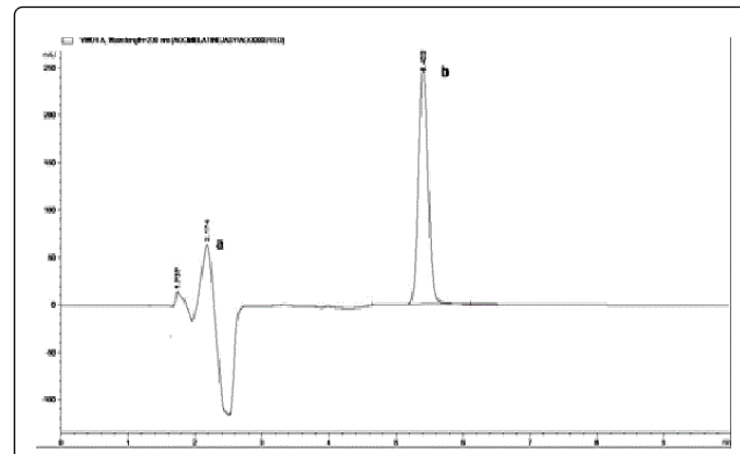
Figure 7: MLC Chromatogram of AGO under optimum chromatographic conditions using Apollo C 18 column (a) solvent front peak (b) AGO peak (5 \mu\text{g}/\text{mL} ).
