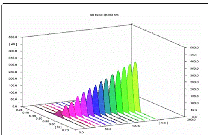
Figure 5: 3D chromatogram of calibration bands of AGO (0.3-4 \mu\text{g} /spot) at 280 nm by RP-TLC.
