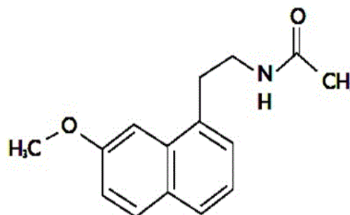
Figure 1: Chemical structure of Agomelatine.
