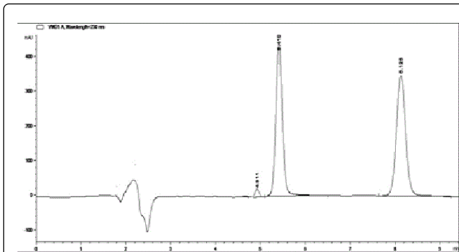
Figure 12: Alkali forced degradation chromatogram of AGO by MLC method.
