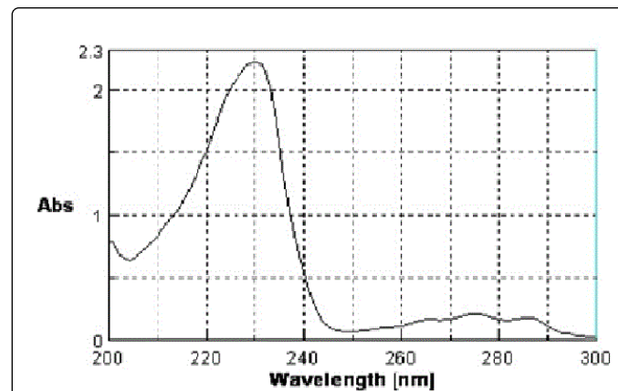
Figure 6: Absorption spectrum of AGO in MeOH.
