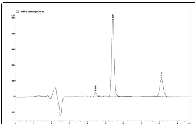
Figure 11: Acid forced degradation chromatogram of AGO by MLC method.
