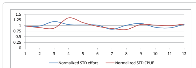
Figure 3: Plot of normalized effort and CPUE based on the 2014 NFIS catch/effort data.
