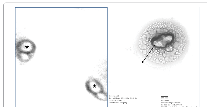
Figure 1: TEM analysis of Alcaligenes sp. membrane vesicle after negative staining. TEM analysis of Alcaligenes sp. after 48 h of inoculation. Asterisk represents large PHB granules. Alcaligenes cell filled with granules. Arrows point to intracellular granules present inside membrane vesicle. Arrow represented the large PHB granule inside the vesicle (magnification 100 nm).
