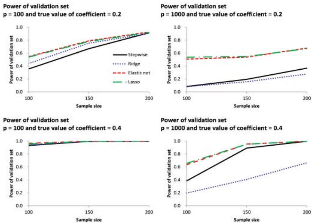
Figure 2: Statistical power of the validation set for the stepwise method and each penalized method using uncensored data sets. Numbers of candidate genes p = 100 and 1000 , and true values of the coefficients = 0.2 and 0.4 .
