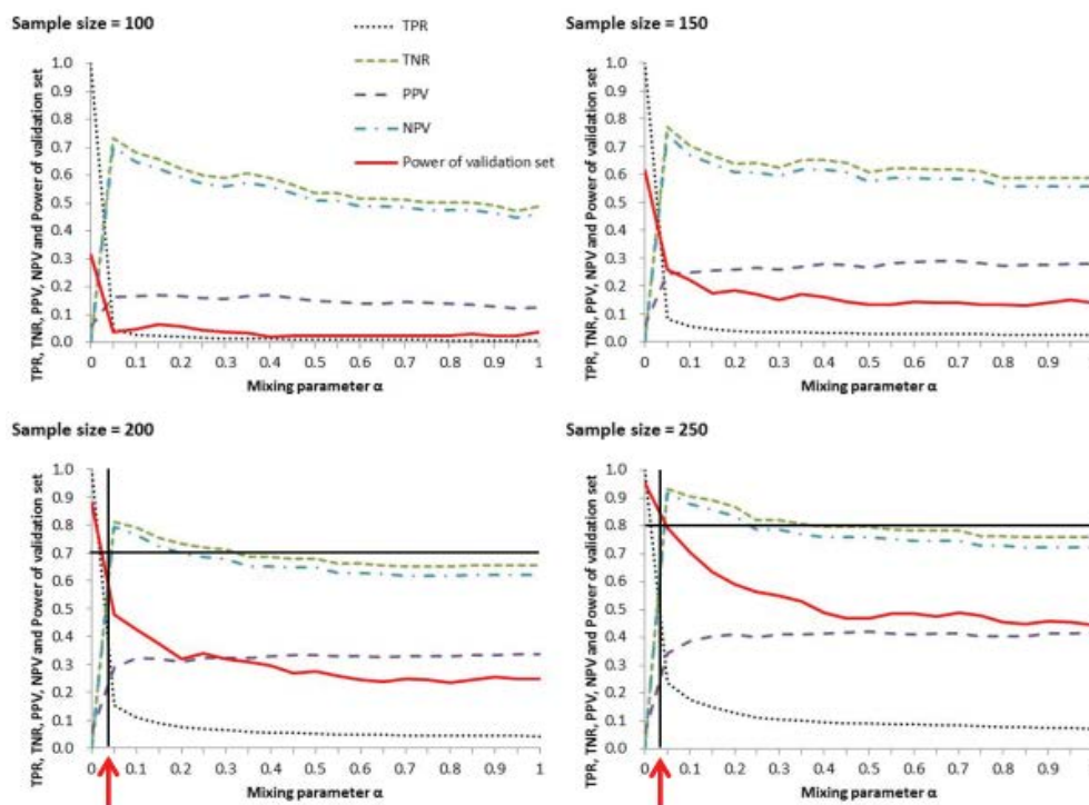
Figure 6: Statistical power and TPR, TNR, PPV, and NPV of the validation set for the penalized Cox's proportion hazard model using actual microarray data sets for ovarian cancer with mixing parameter \alpha . The red arrow indicates \alpha values under 0.05 can detect coefficients of 0.7 or larger with at least 80% power at the 5% significance level.
