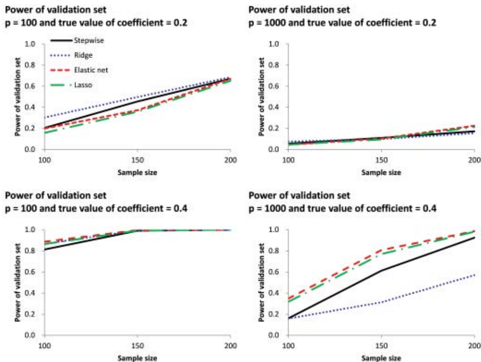
Figure 4: Statistical power of the validation set for the stepwise method and each penalized method using censored data sets. Numbers of candidate genes p = 100 and 1000 , and true value of the coefficients = 0.2 and 0.4 .
