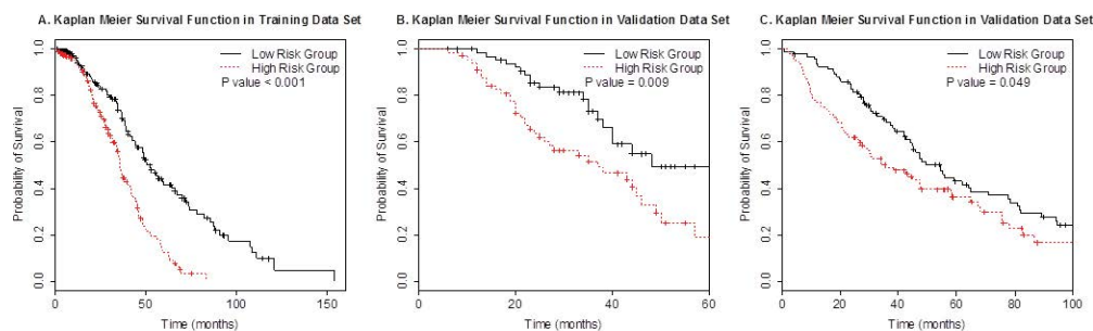
Figure 7: Verification of the validity of the penalized Cox's proportional hazards model using actual microarray survival data. Three actual microarray data sets for ovarian cancer were used. A. The cancer genome atlas (TCGA) data set [6] was used as the training data set; B. Tothill's data set [7] was used as a validation data set; and C. Bonome's data set [8] was used as a validation data set.
