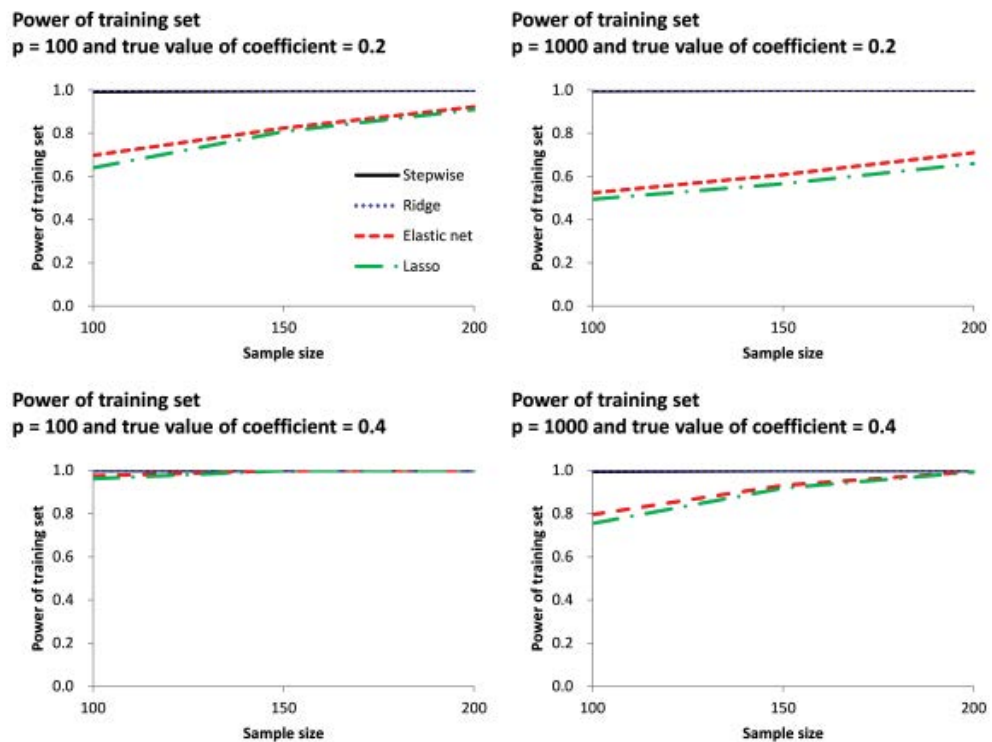
Figure 3: Statistical power of the training sets for the stepwise method and each penalized method using censored data sets. Numbers of candidate genes p = 100 and 1000 , and true value of the coefficients = 0.2 and 0.4 .
