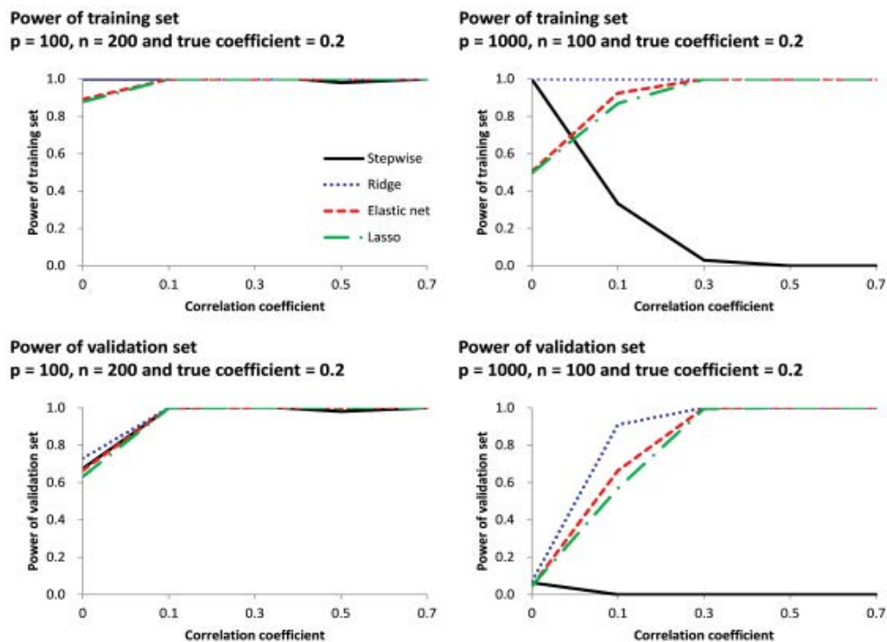
Figure 5: Statistical power of the training and validation sets for the stepwise method and each penalized method using censored data sets with correlation coefficients. When the numbers of candidate genes p = 100, n = 200 ( n > p ; first column), and when p = 1000, n = 100 ( n < p ; second column), and true value of the coefficient = 0.2 .
