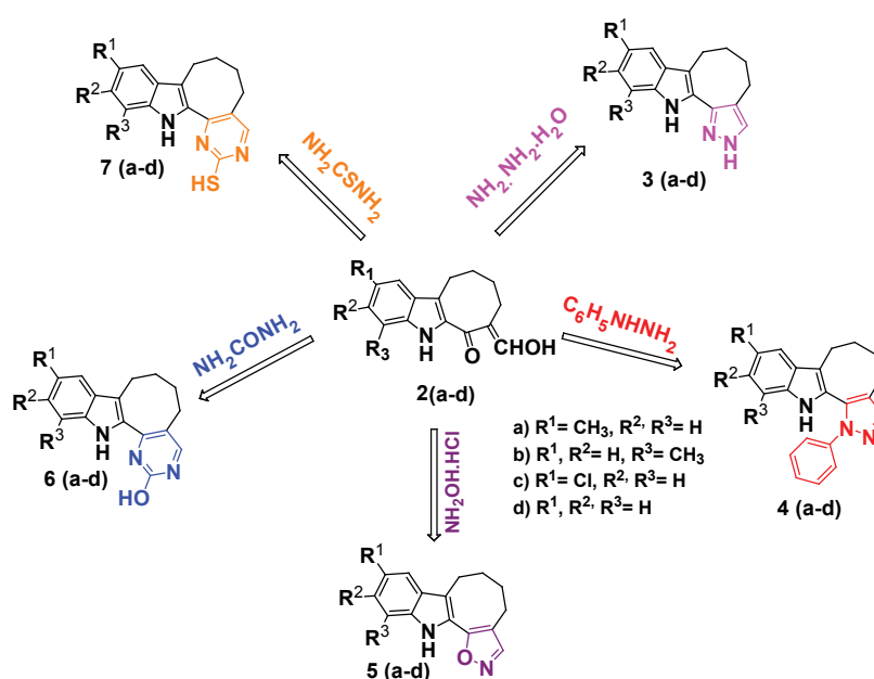
Scheme 2: Synthesis of isoxazolo-, pyrido- and pyrazolo-cycloocta[b]indoles.
