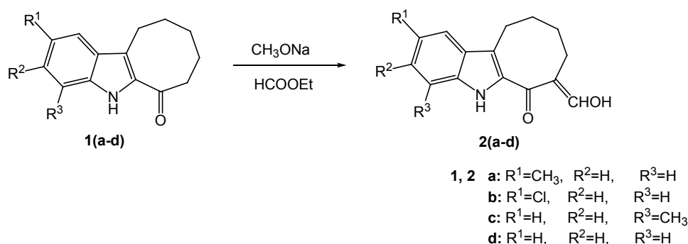
Scheme 1: Synthesis of 7-(hydroxymethylene)-5,7,8,9,10,11-hexahydrocycloocta[b]indol-6-ones.
