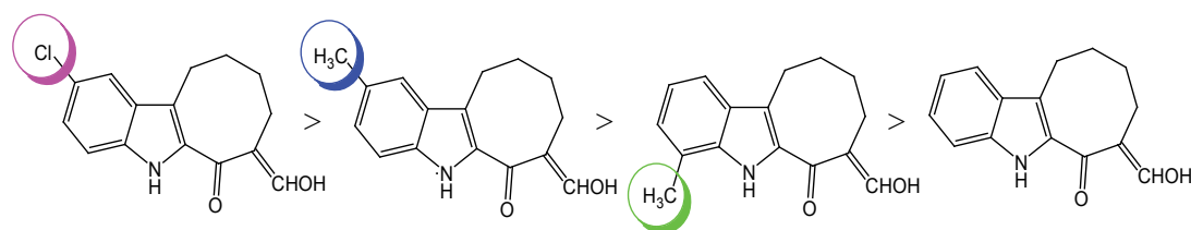
Figure 2: The decreasing order of activity of intermediates.
