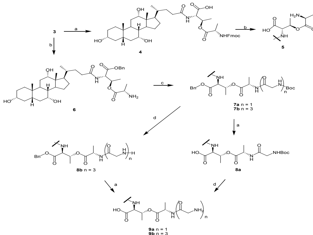
Scheme 3: Reagents and condition: (a) H 2 , 10% Pd/C, methanol, room temperature; (b) KF, TEA, DMF (or piperidine), DCM r.t.; (c) DCC, peptides or protected amino acids, DMAP (or TEA), DMF/THF; (d) 55% trifluoroacetic acid (TFA) in DCM, r. t..
