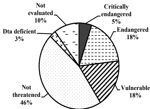
Figure 3: Conservation status of SIS under different categories.
