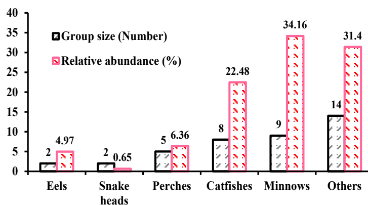
Figure 4: Size and relative abundance of common groups of SIS.
