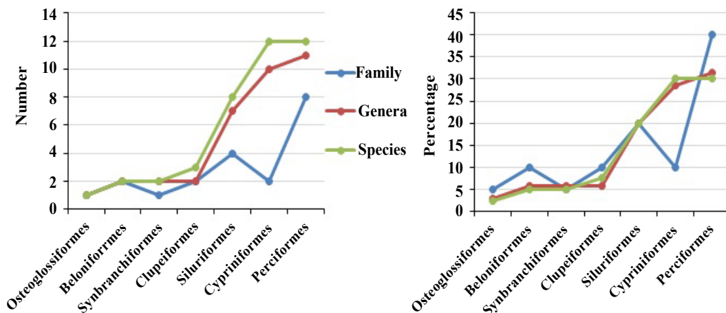
Figure 2: Number and percent composition of families, genera and species of SIS under various orders recorded in the Gorai River.
