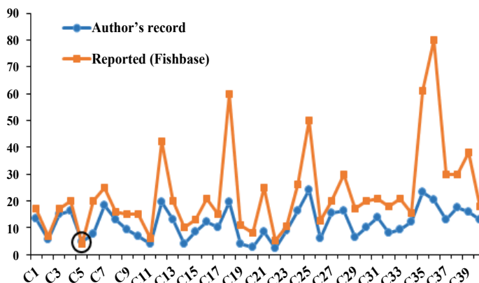
Figure 5: Maximum total length of SIS of collected sample by author vs. reported total length.
