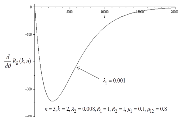
Figure 11: Sensitivity of system reliability with respect to \lambda_1 .
