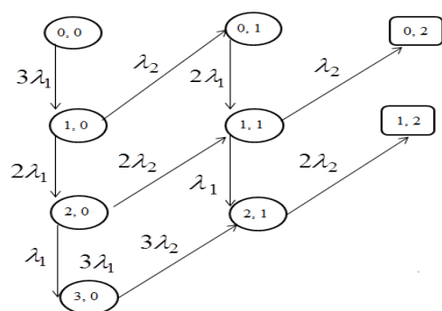
Figure 2: TMR with degradation diagram.
