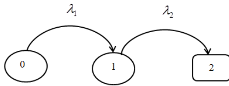
Figure 1: Simplex system with degradation diagram.
