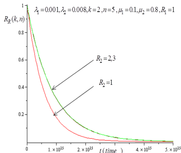
Figure 9: Repairable system reliability for different numbers of repairmen in second service line.
