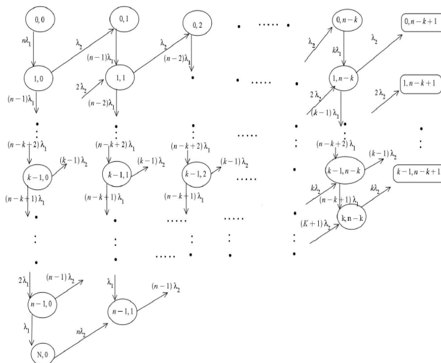
Figure 3: State-transition-rate diagram of non-repairable System with degradation.
