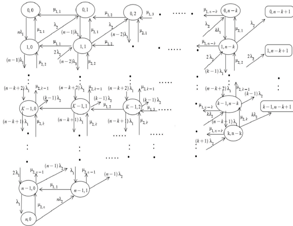
Figure 7: State-transition-rate diagram of repairable System with degradation facility.
