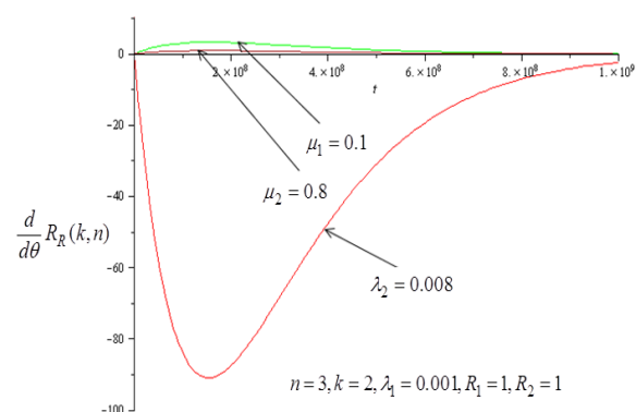
Figure 10: Sensitivity of system reliability with respect to \lambda_2 , \mu_1 and \mu_2 .
