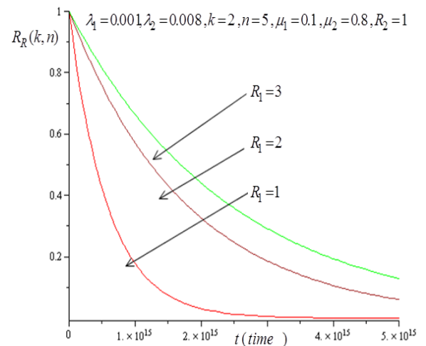
Figure 8: Repairable system reliability for different numbers of repairmen in first service line.
