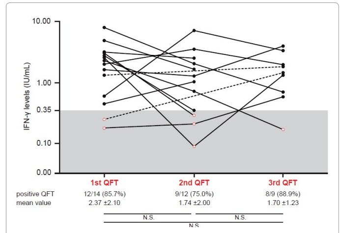
Figure 1: The change in IFN- \gamma level in patients with active pulmonary tuberculosis.
