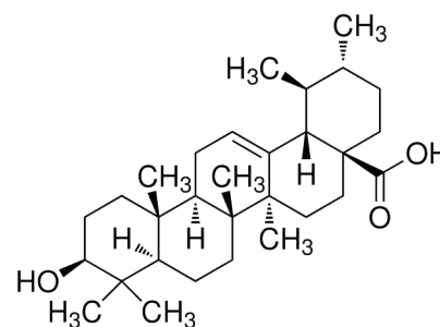
Figure 1: Chemical structure of UA.
