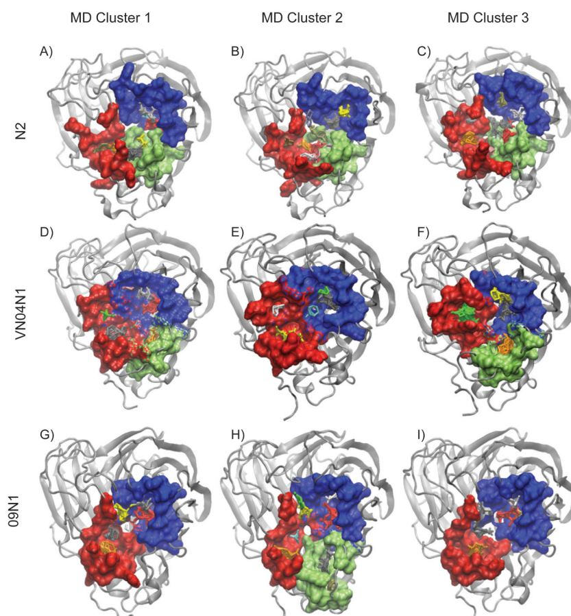
Figure 2. Neuraminidase hot spots. Ligand- and receptor-binding hot spots are shown for the sialic acid cavity (blue), 150-cavity (green), and secondary sialic acid and 430-cavities (red) for the most predominant N2 (A), second most predominant N2 (B), third most predominant N2 (C), most predominant VN04N1 (D), second most predominant VN04N1 (E), third most predominant VN04N1 (F), most predominant 09N1 (G), second most predominant 09N1 (H), and third most predominant 09N1 (I) ensemble structures. Clusters of organic probes indicating actual hot spot/probe binding locations are shown in various colors in stick representation.
