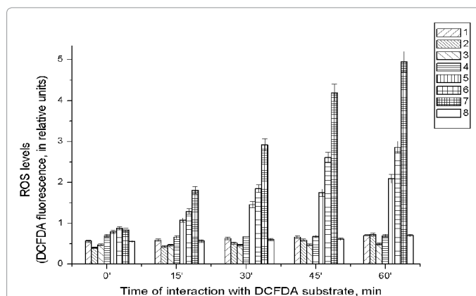
Figure 7: The level of ROS/RNS production in E. coli TN530 cells treated with 0.05 mM TNIC thio and PABA influence: 1-control; 2-menadione 0.5 mM; 3-PABA 5 mM; 4-TNIC thio +PABA 5 mM; 5-TNIC thio +PABA 0.5 mM; 6-NIC thio +PABA 0.05 mM; 7-TNIC thio 0.05 mM; 8-CF 0.05 mM. The levels of all samples are indicated by deducing «0» for PBS fluorescence.
