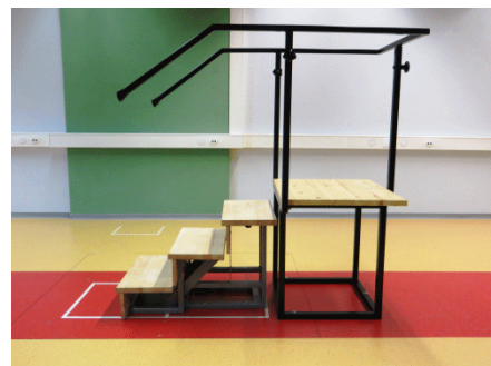
Figure 1: Photograph of the stairway set-up on the force plates. The stairway was attached with threaded inserts on the platforms. The stairway allows for measuring isolated forces and moments generated during each of four consecutive steps.
