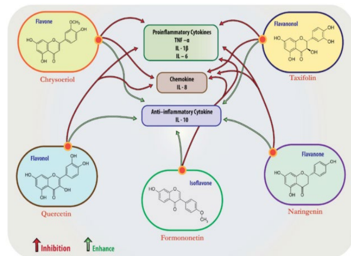
Figure 2: Possible anti-inflammatory inhibition mechanism of flavonoids from P. daemia .
