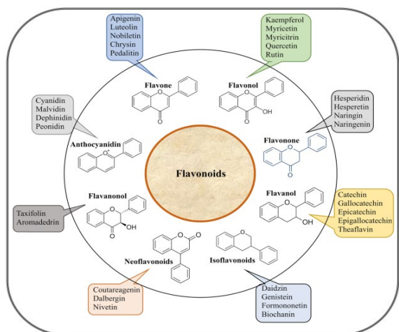
Figure 1: Basic skeleton of flavonoids and its subgroups.
