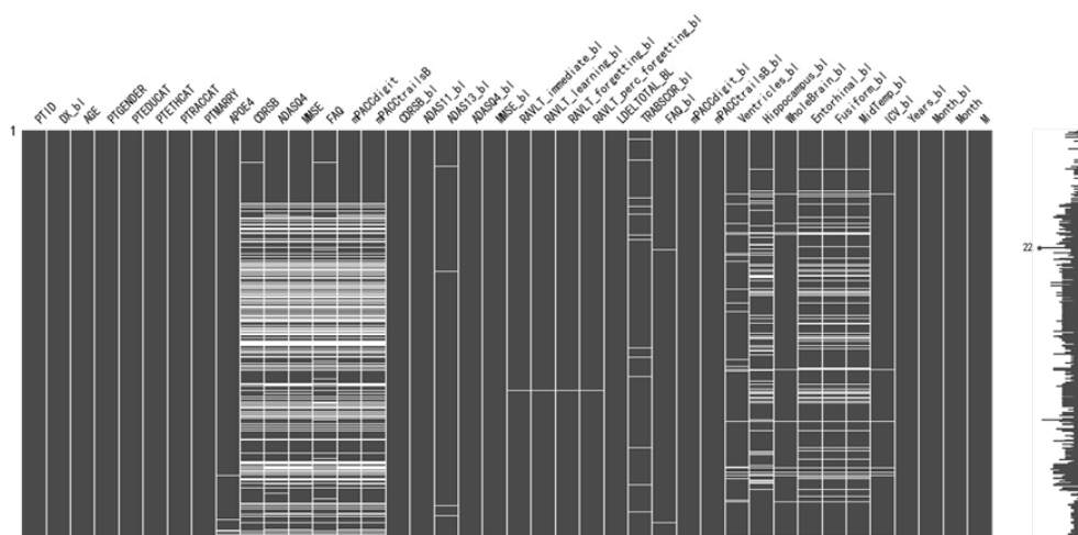
Figure 4: Distribution of missing values of processed data.
