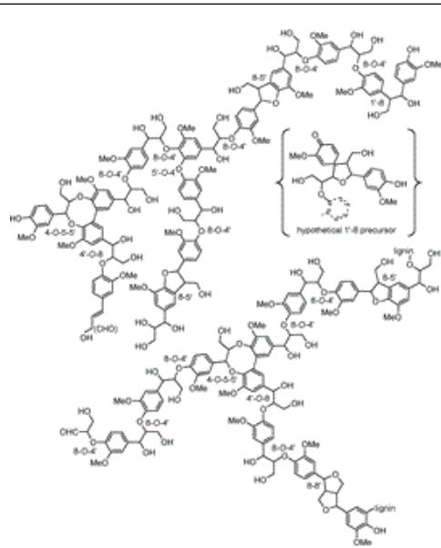
Figure 1: An exemplary segment of softwood lignin.
