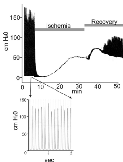
Figure 2: Condensed pressure tracing generated using a silicone balloon inserted into a mouse heart that was made ischemic for 25 minutes and then unclamped and allowed to recover. The spontaneous beat rate in this example was 360 \pm 23 bpm.
