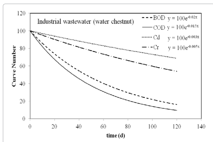
Figure 5: Variation of Curve Number (CN) with time (days).
