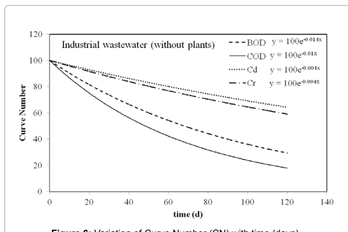
Figure 6: Variation of Curve Number (CN) with time (days).
