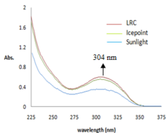
Figure 5: UV spectrum of lamotrigine.
