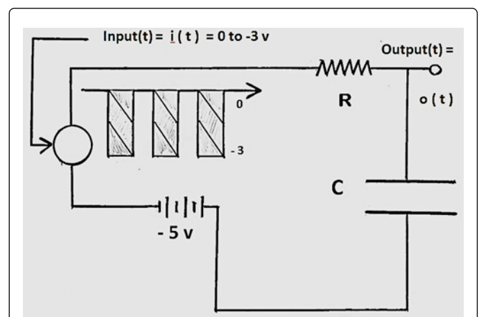
Figure 1: Electrical circuit shows the refractive development as the voltage at the capacitor of a corrected -5 D eye, periodically reading at a distance of 1/3 meter (14 inches).
