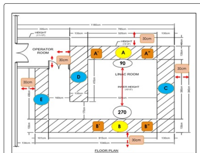
Figure 2: Figure showing floor plan of radiation therapy bunker with barriers and points of measurements.
