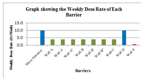
Figure 6: Chart showing Weekly Dose Rate of the Barriers.
