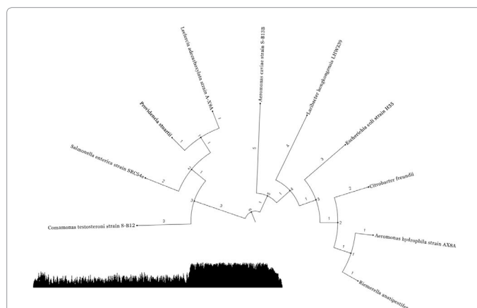
Figure 2: Phylogenetic reconstruction of aadA1 aminoglycoside resistance genes. Taxa order (inner-node to outer-node arrangement): clade a) Leclercia adedecarboxylata A-X9A, Providencia stuartii , Salmonella enterica SRC54e, Comamonas testosteroni S-B12; clade b) Riemerella anatipestifer , Aeromonas hydrophila AXBA, Citrobacter freundii , Escherichia coli H35, Laribacter hongkongensis LHW339, Aeromonas caviae S-B13B.
