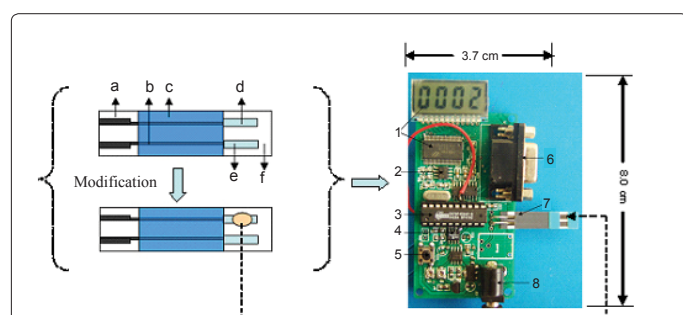
Figure 1: Schematic diagram of the SPE and components of the hardware of the amperometric sensor. The schematic structure of SPE consisted of following parts: (a) terminal post, (b) electric conductive rail, (c) insulation layer, (d) working electrode, (e) counter electrode and (f) polyvinyl chloride board. The hardware components of the amperometric sensor: (1) liquid crystal display and HT1621 driving chip, (2) MCP3201 A/D converter, (3) EM78P458 single-chip microcomputer, (4) operational amplifier, (5) function key, (6) data-interface, (7) SPE slot and (8) battery (output, 6 V).
