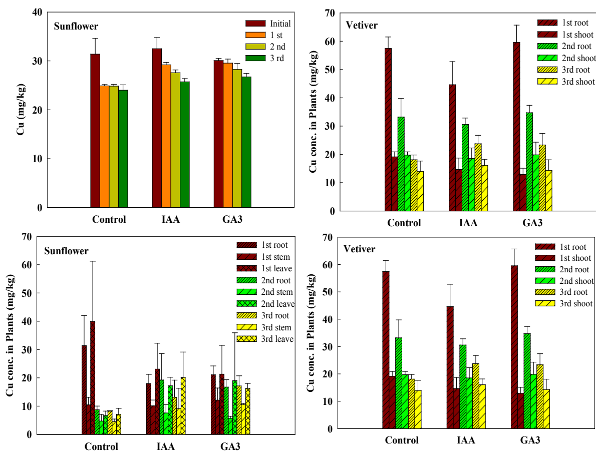
Figure 2: Cu concentration (mg/kg) in different parts of vetiver and sunflower.
