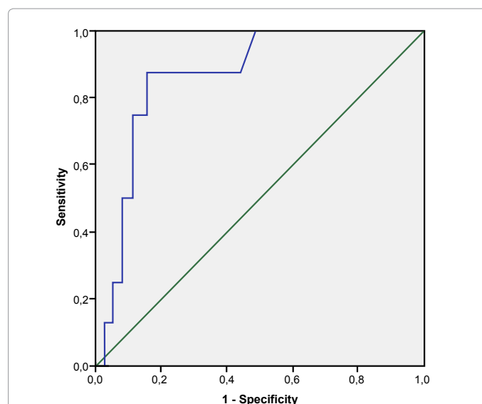
Figure 2: ROC Curve FEV 0.75 /FVC. Area under the curve: 0.860 ± 0.440 (95% CI: 0.775-0.948).
