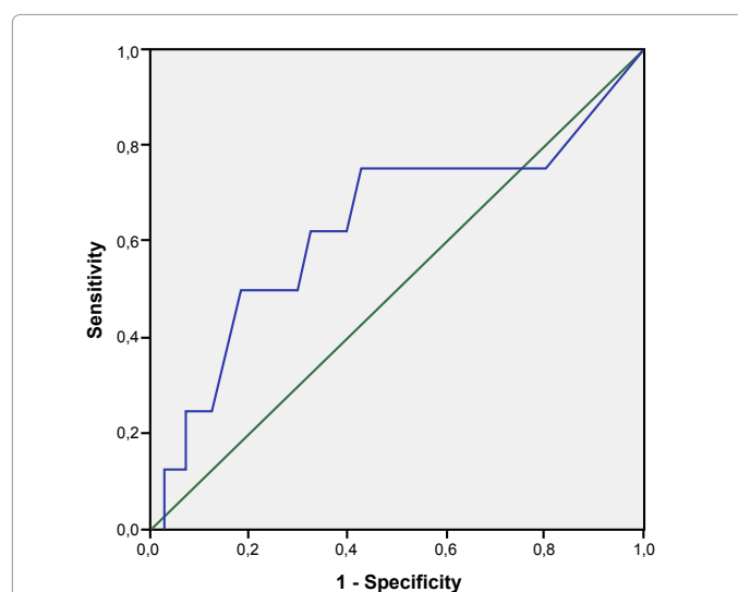
Figure 1: ROC Curve FEV 1 /FVC. Area under the curve: 0.632 ± 0.087 (95% CI: 0.461-0.804).
