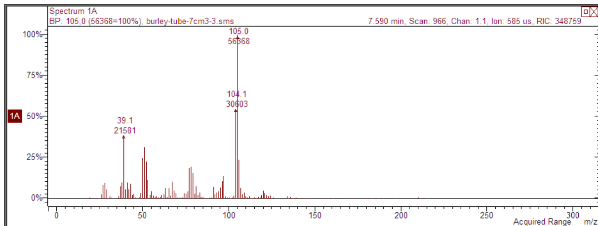
3-ethenyl-pyridine
