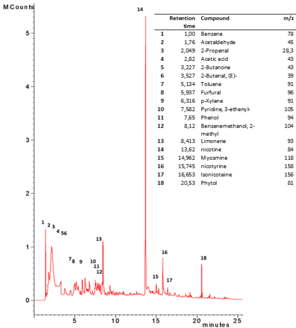
Graph showing all the detection limit peaks of different compounds.
