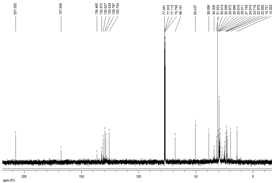
Appendix 8: ^{13}\text{C} NMR Spectrum of CP-4.
