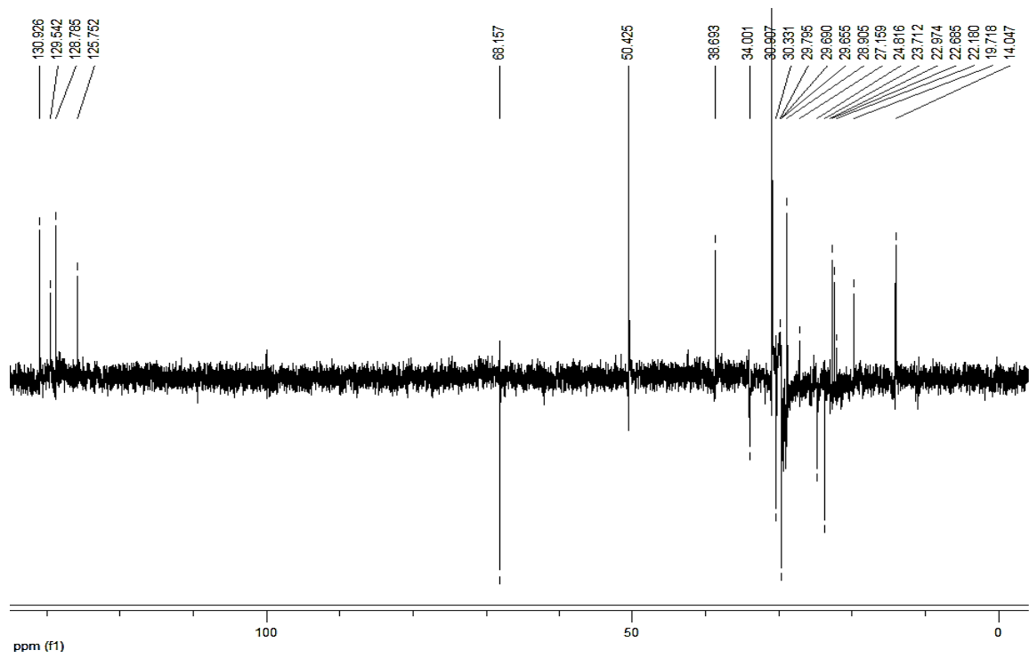
Appendix 9: DEPT-135 NMR Spectrum of CP-4.
