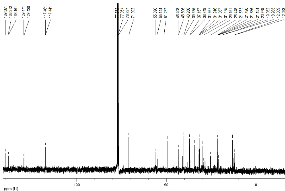
Appendix 4: ^{13}\text{C} NMR Spectrum of CP-1.
