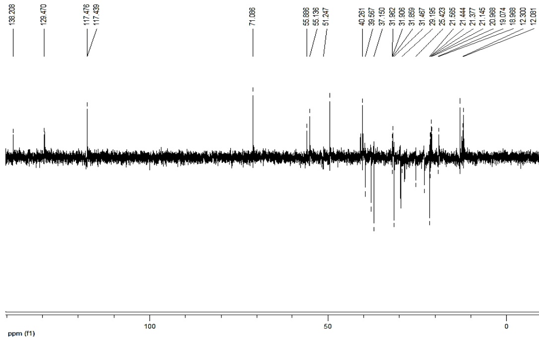
Appendix 5: DEPT-135 NMR Spectrum of CP-1.
