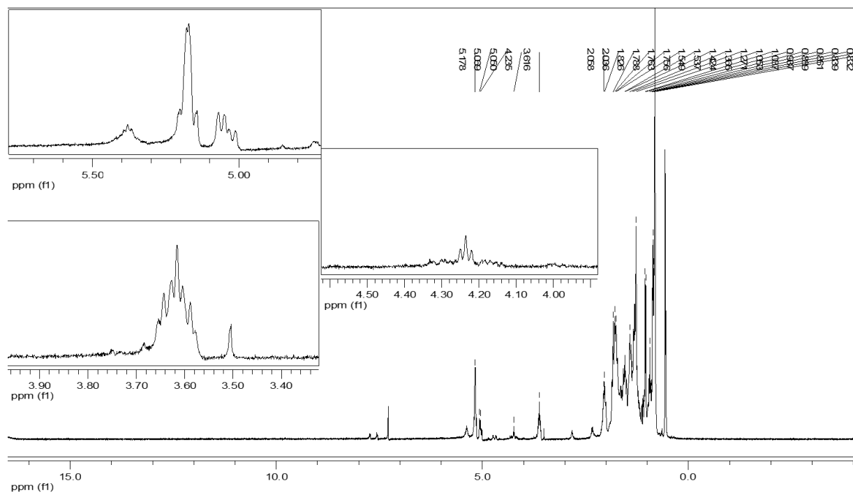
Appendix 3: ^1\text{H} NMR Spectrum of CP-1.
