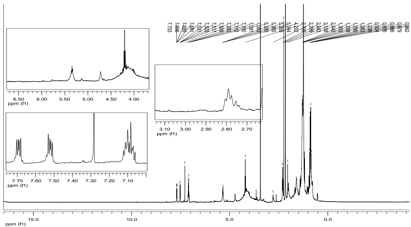
Appendix 7: ^1\text{H} NMR Spectrum of CP-4.
