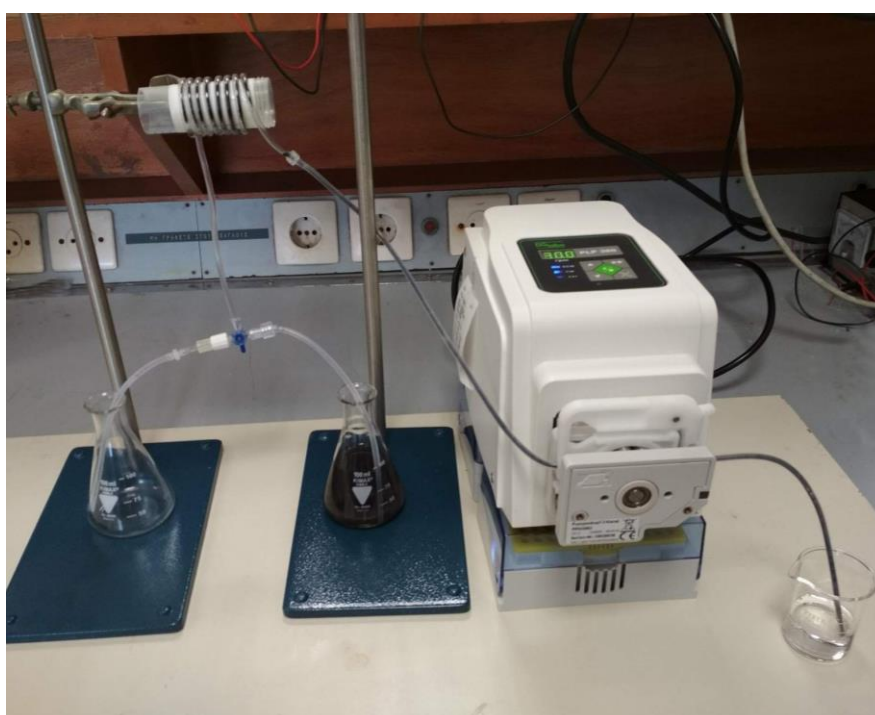
Figure 2: View of the entire apparatus before magnetic particles harvesting.
